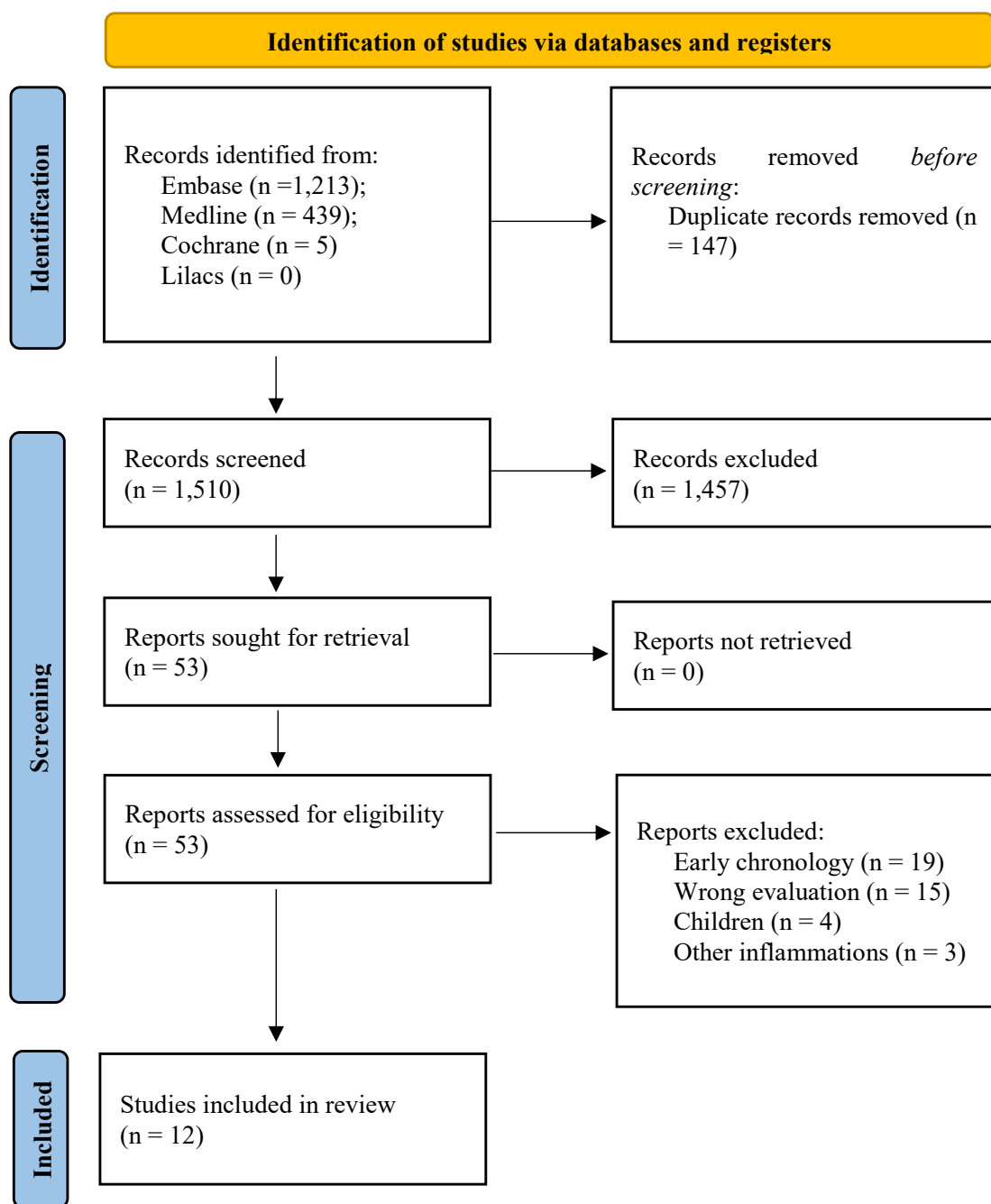
Figure 1 – Prisma flowchart.
