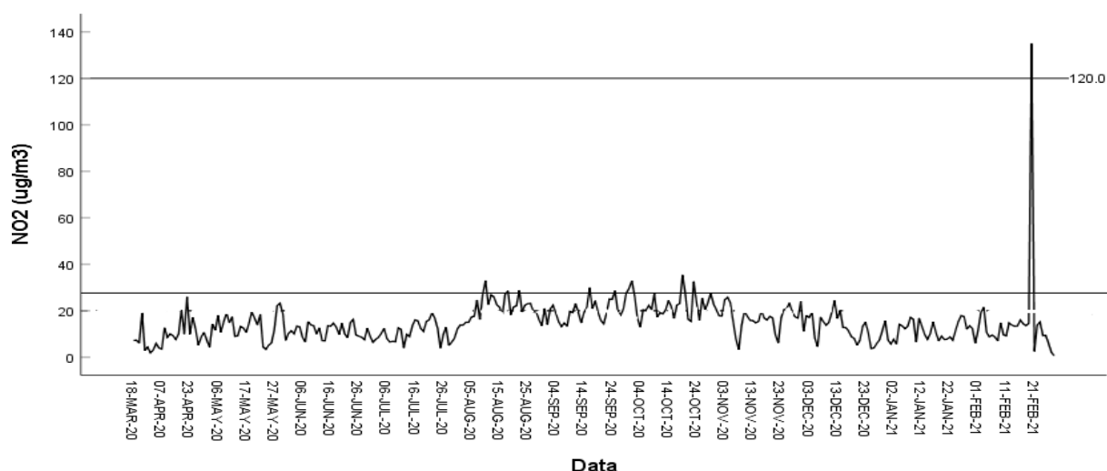
Figure 3 – Average daily concentration of NO 2 in the municipalities of Canoas and Esteio/RS
