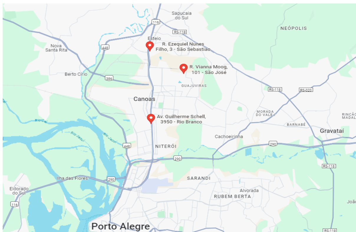
Figure 1 – Location map of automatic air quality stations in the municipalities of Canoas and Esteio/RS
