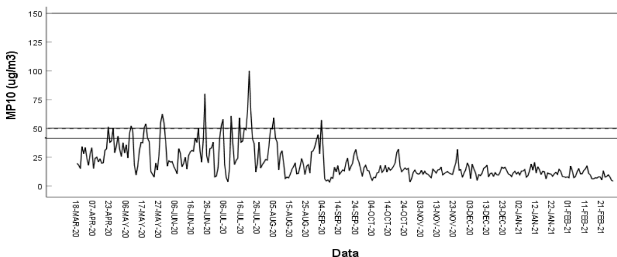
Figure 4 – Average daily concentration of \text{MP}_{10} in the municipalities of Canoas and Esteio/RS
