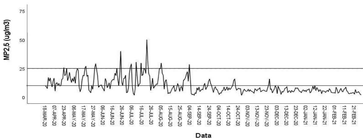
Figure 5 – Average daily concentration of \text{PM}_{2.5} in the municipalities of Canoas and Esteio/RS
