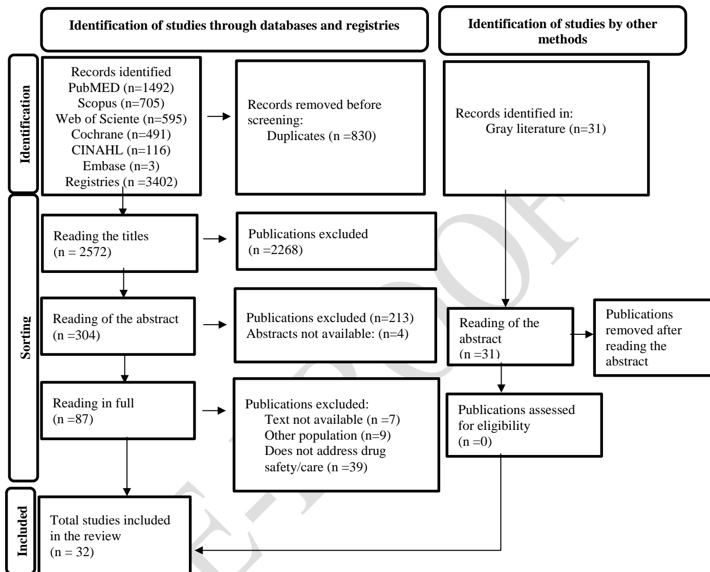
Figure 1. Flowchart adapted from the Prisma Extension for Scoping Reviews (Primas-ScR) 10 , which was used to select safety studies on nursing care in the preparation and administration of sedative, analgesic and vasoactive drugs in critically ill patients.
